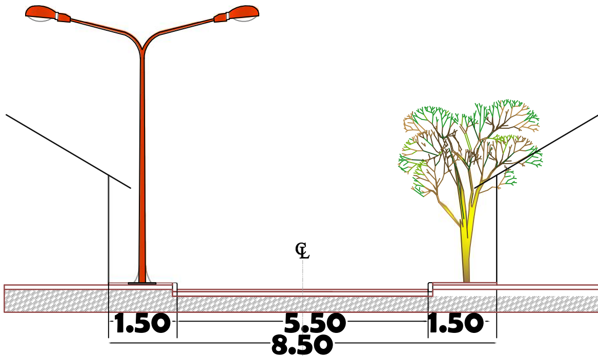
VIA BARRIAL ESC: 1 _____ 200
